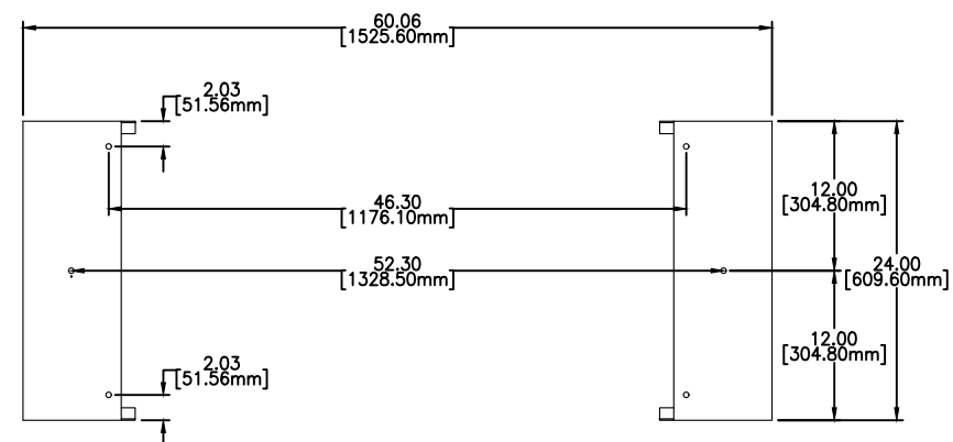
LEG STAND KIT MOUNTING
