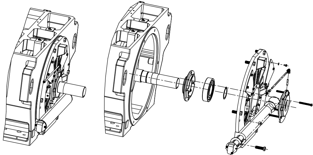
Figure 7. Drive End and Opposite Drive End Bearing Assemblies.
