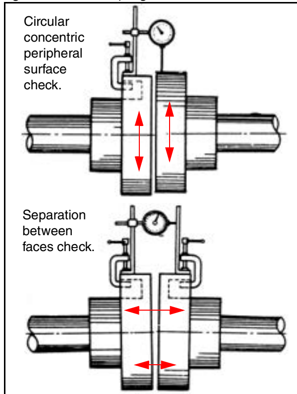
Figure 3. Direct Coupling Checks.
