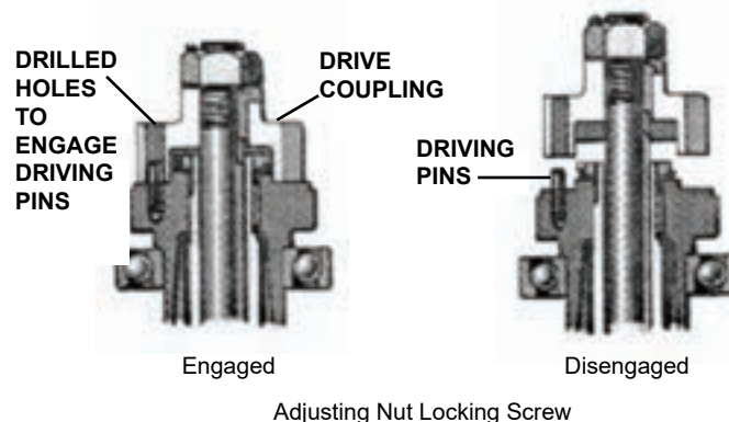
Figure 4 Self Release Coupling
